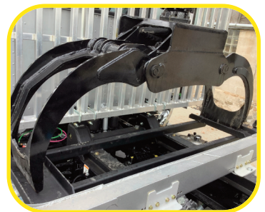
Bolt on bucket/grapple carrier
