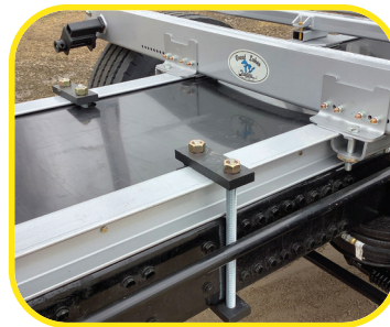
Subframe tie down and bunk clamping systems
